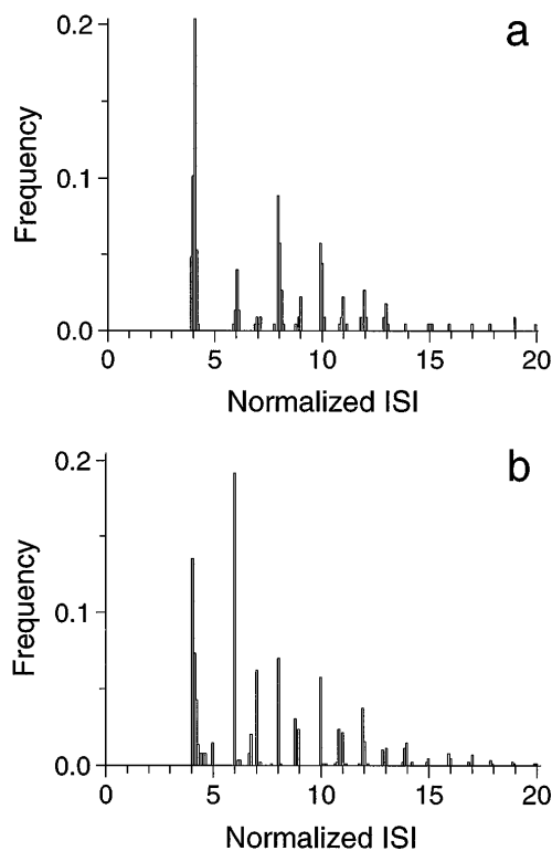
FIG. 4. Interspike interval (ISI) histograms from squid axon and FitzHugh-Nagumo model. (a) Squid axon: data taken from the run, part of which is shown as Fig. 1(g) ( T = 12.2 ms). (b) FitzHugh-Nagumo model: data taken from simulations of Fig. 3 ( T = 29.5 time units). In both (a) and (b), intervals are calculated between peaks of action potentials and are normalized to the interstimulus interval.
