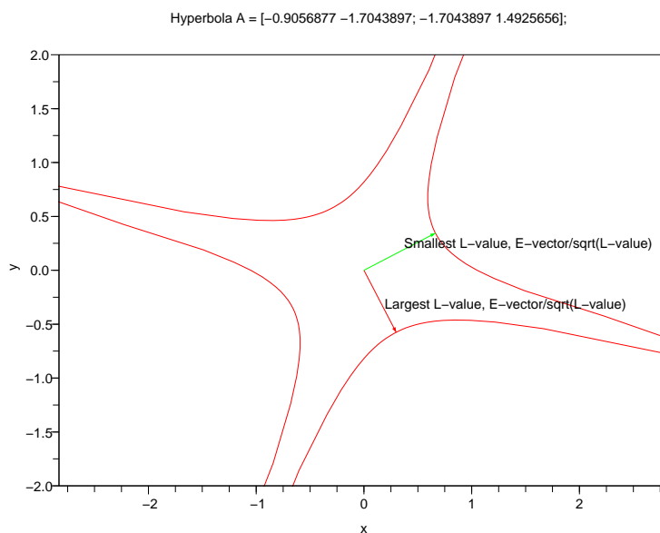
FIGURE 1. X^T A X = 1 and E-vectors/L-values of Hyperbolic Example
