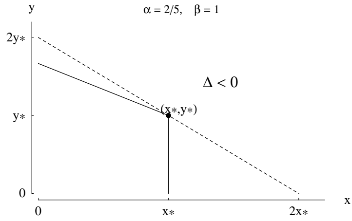
Figure 17.3 Why u^* is evolutionarily stable
