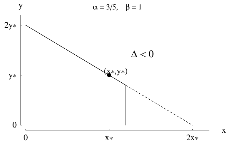
Figure 17.4 Why u^* is evolutionarily stable
