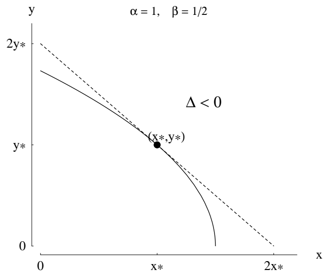
Figure 17.2 Why u^* is evolutionarily stable
