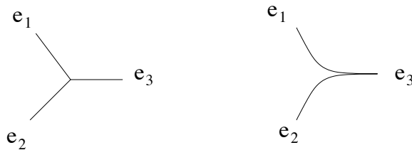
FIGURE 5. Smoothing at a trivalent vertex
