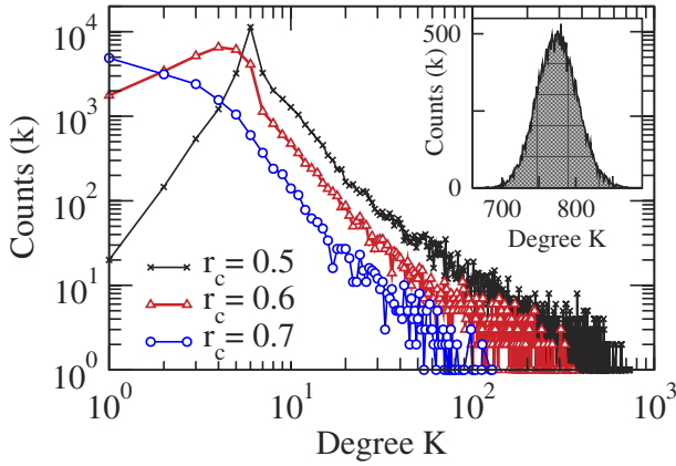
FIG. 2 (color online). Degree distribution for three values of the correlation threshold. The inset depicts the degree distribution for an equivalent randomly connected network.
