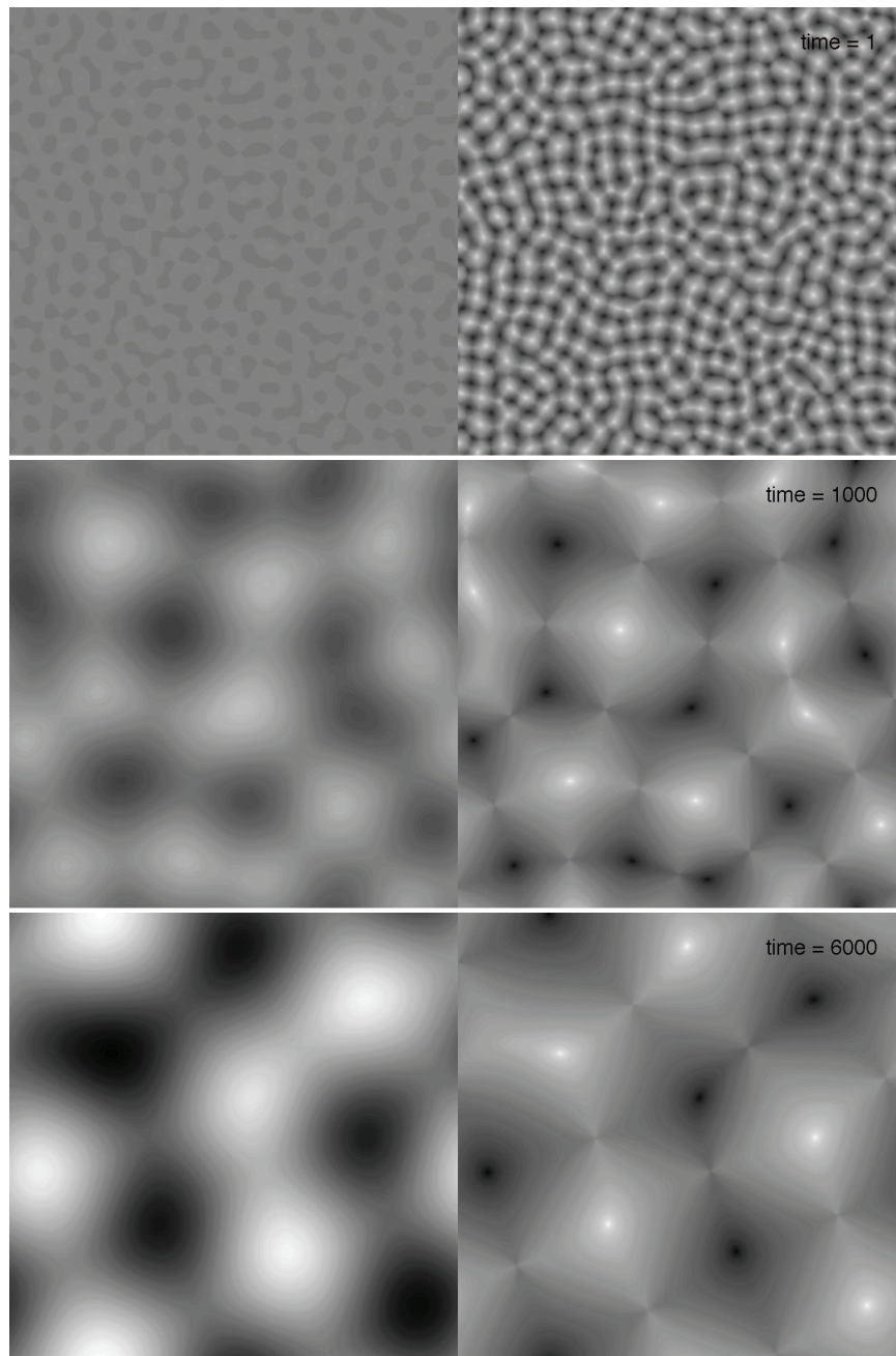
FIGURE 3. Time snapshots of the evolution of the model without slope selection. The plots are as in Fig. ??, with \phi on the left-hand-side and \Delta\phi on the right-hand-side. The system does not saturate by time 6000.
