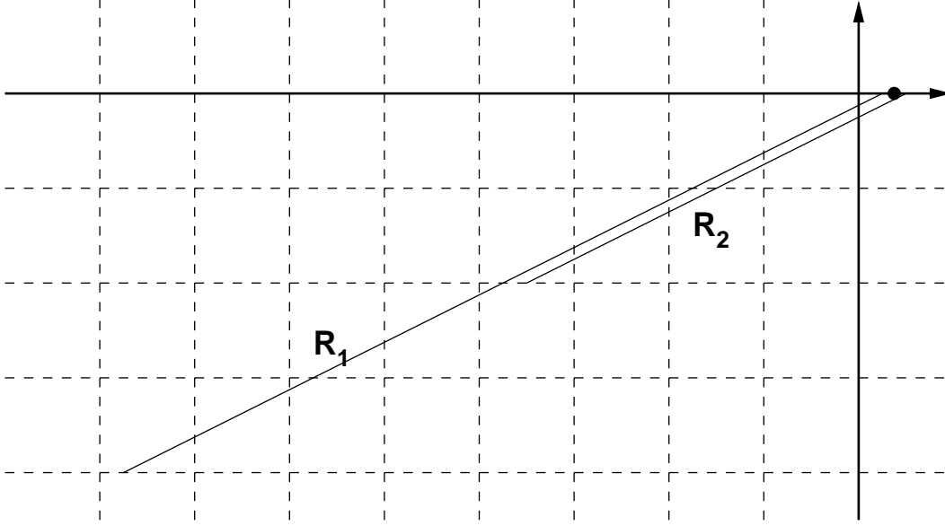
FIGURE 9. +\frac{1}{2} surgery on K(2, 5)
