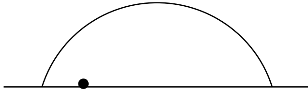
FIGURE 4. SU(2) representations of the trefoil.
