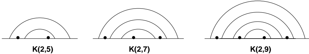
FIGURE 7. SU(2) representation varieties of (2, q) torus knot groups
