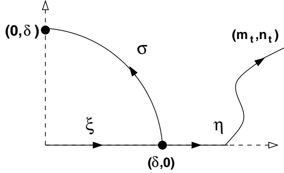
FIGURE 2. The paths \xi , \eta , and \sigma
