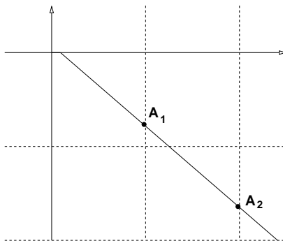
FIGURE 6. Two flat connections extending over \Leftrightarrow 1 surgery on the right hand trefoil
