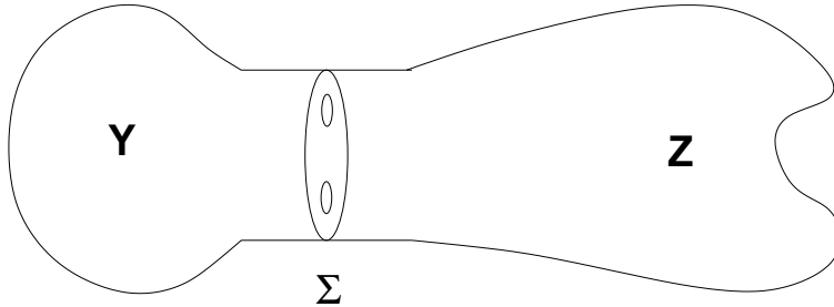
FIGURE 1. The split 3-manifold X
