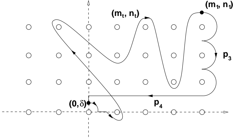
FIGURE 3. The loop \ell and numbers a = 4 , b = 3 and c = \Leftrightarrow 2(1 \Leftrightarrow 9) = 16 .
