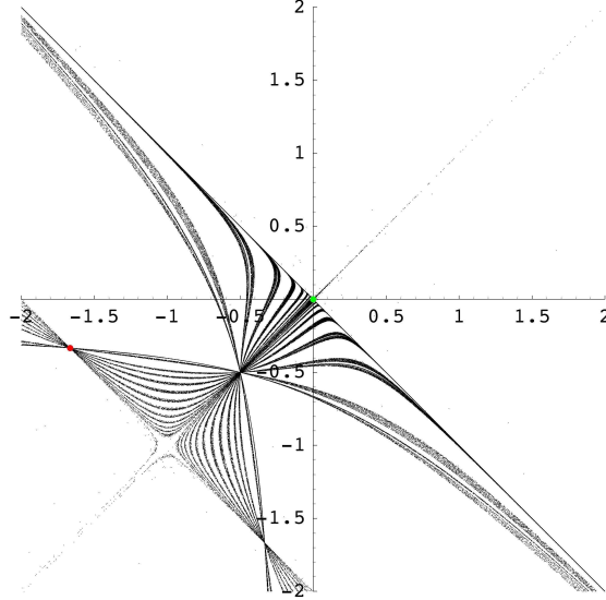
Figure 6.1. An Exceptional Orbit: q = 12 .
