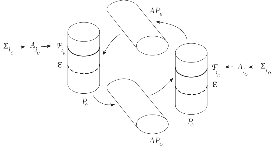
Figure 5.1. Exceptional Orbits: The Wringer.
