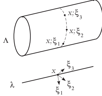
Figure 1.1. Blowup of a Linear Subspace.
