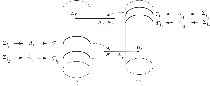
Figure 4.1. Exceptional Orbits: Hooks.
